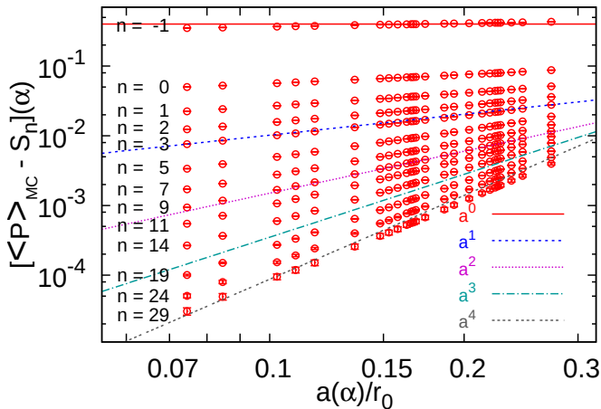
Figure: \langle P \rangle_{MC}(\alpha) - S_n(\alpha) between MC data and sums truncated at orders \alpha^{n+1} ( S_{-1} = 0 ) vs. a(\alpha)/r_0 . The lines \propto a^j are drawn to guide the eye.
