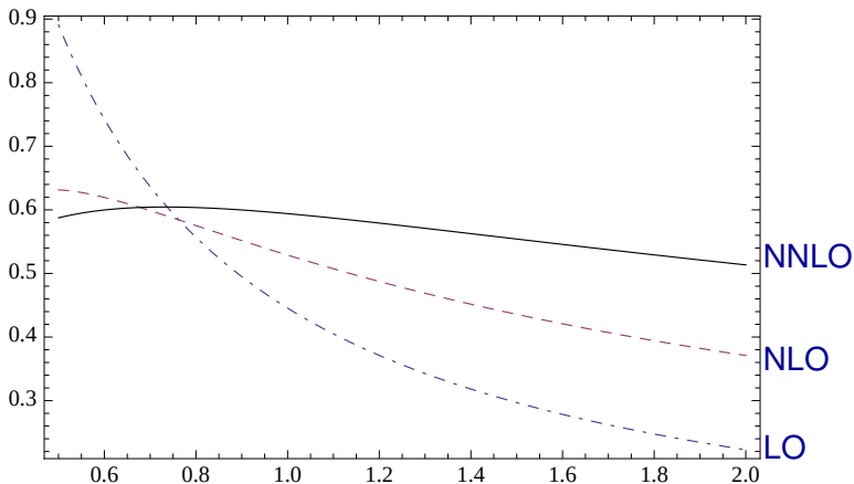
Figure: N_m for n_l = 3 , as a function of x \equiv \mu/m_b , obtained from r_n/r_n^{asym} with r_n^{asym} truncated at \mathcal{O}(1/n^3) . We name the different lines as NNLO (solid), NLO (dashed) and LO (dashed-dotted) for n = 0, 1, 2 , respectively.
