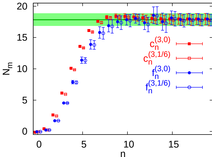
Figure: N_m^{latt} determined via r_n truncated at NNNLO, from the coefficients c_n^{(3,0)} , c_n^{(3,1/6)} , f_n^{(3,0)} and f_n^{(3,1/6)} . The horizontal band is our final result: N_m = 17.9(1.0)
