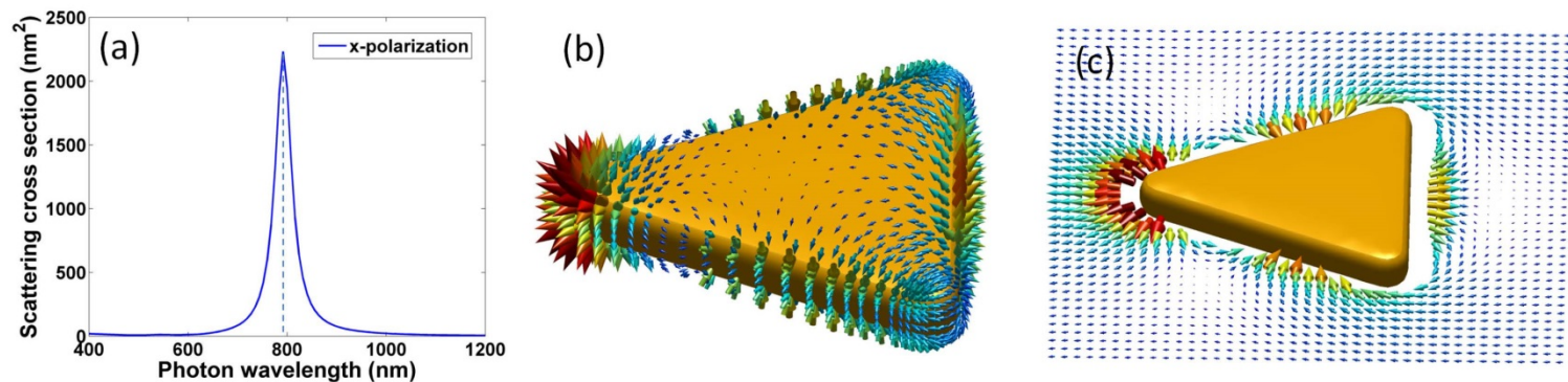
Figure 4.4.: (a) Scattering cross section of a gold nanotriangle ( 55 \times 50 \times 8 \text{ nm} , n_b = 1.34 ). The panels (b) and (c) show the electric field at the resonance energy of 792 \text{ nm} at the particle surface and on the outside, respectively. (Also see Fig. 3.7.) A. Trügler, PhD thesis (2011)
